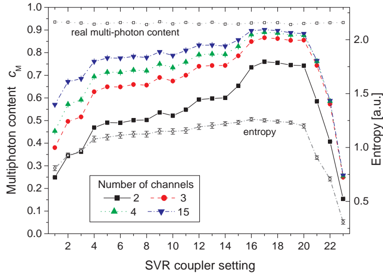
Fig. 4. Dependence of the multi-photon content c_M on the SVR setting when detected 2, 3, 4 or 15 channels of the device (see inset legend). A real multi-photon content in the coherent state in front of the device (dotted line with open rectangles) is shown for comparison. The mean pulse energy \mu of the input state was 4.26 photons per pulse. The dash-dot line with open circles is Shannon entropy computed from measured division ratios of the first 15 channels.
